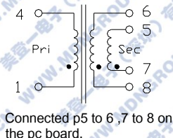
SCHEMATICS
