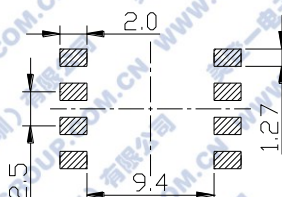
LAND PATTERN
